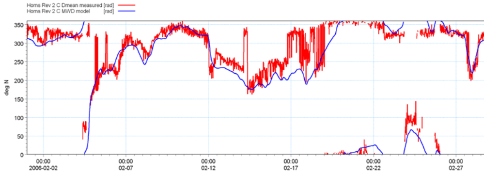
Figure 9 Comparison of mean wave direction from wave model (blue) and measurements (red) at Centre
